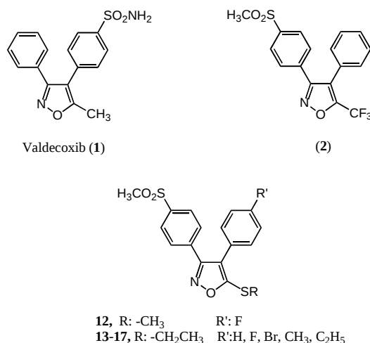
Representative examples and designed 3,4-diarylisoxazoles as COX-2 selective inhibitors.
